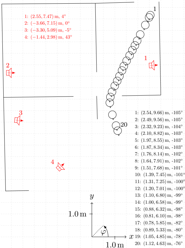
Loudspeaker and KEMAR positions
